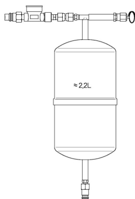
Figure 1: The figure shows an example of a test storage bottle with a high side and low side connection (and one connection for the creation of pressure to test the discharge of non-condensable gases) with a volume of 2.2 litre.
