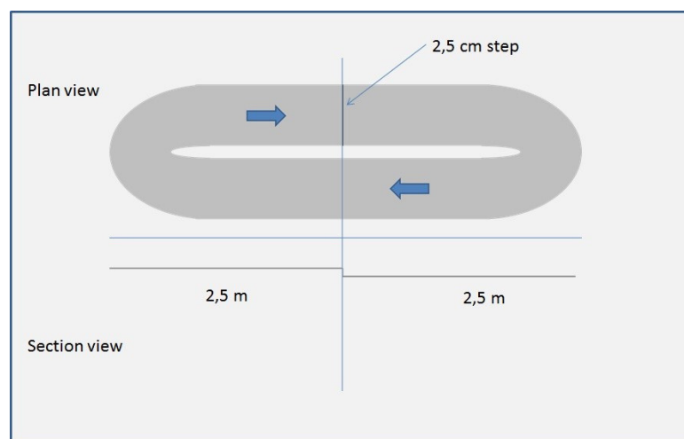
Figure 2 – Scale accuracy reliability test
